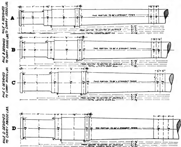
Figs. 4878-4881. Standard Axles. Plate 1.
